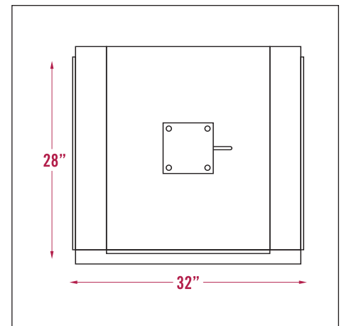
OVERHEAD VIEW
