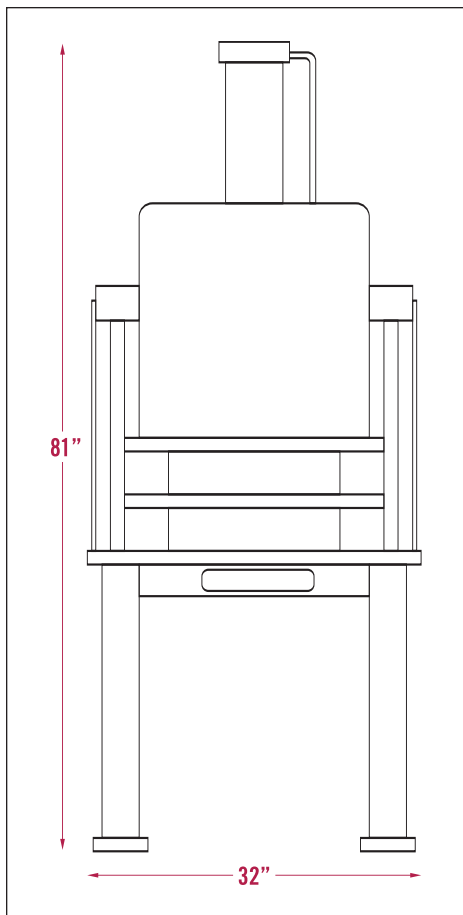
DIMENSIONS: FRONT VIEW
