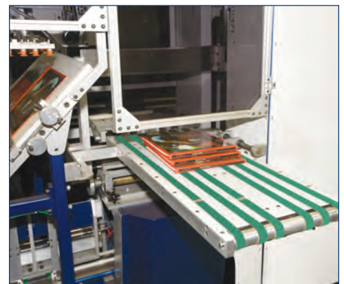
Cased-in hard cover books come off right conveyor belt. Auto-feed attachment for Super Smasher™ available.
