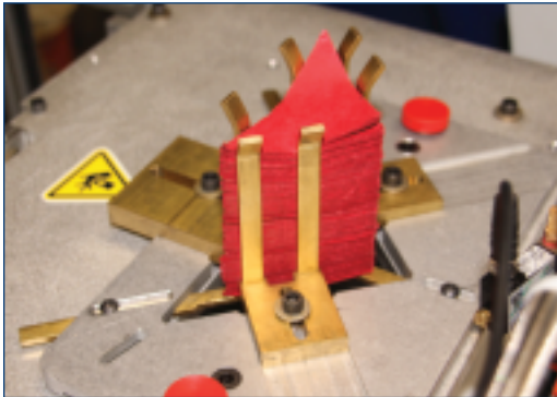
Top loading hopper stacks and pre-aligns corners. Holds up to 200 die cut corners.
