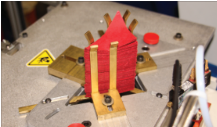
Top loading hopper stacks and pre-aligns corners. Holds up to 200 die cut corners.
