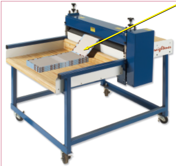
Built-in catching basin neatly stacks finished straightened covers
